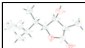
Fig. 1. : The molecular structure of molecule one of (I), with displacement ellipsoids for the non-hydrogen atoms shown at the 30% probability level.
