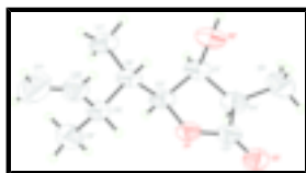
Fig. 2. : The molecular structure of molecule two of (I), with displacement ellipsoids for the non-hydrogen atoms shown at the 30% probability level.
